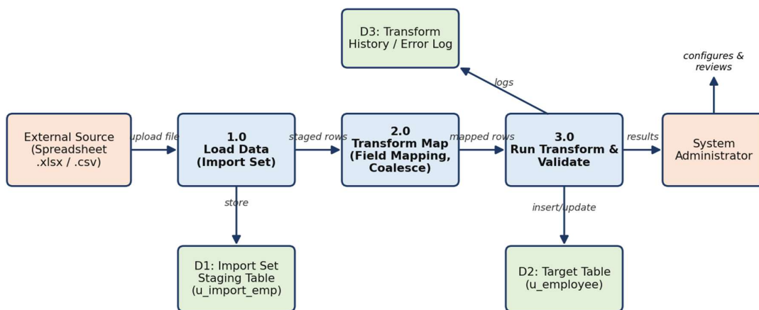
Data Flow Diagram - Import Data using Transform Maps (Spreadsheet)
